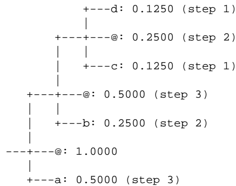
Figure 5.1 Huffman Tree: Entropy equal average code length.
