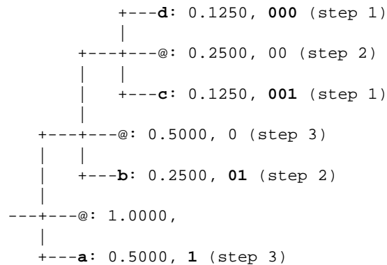
Figure 5.2 Huffman Tree: Codewords.
