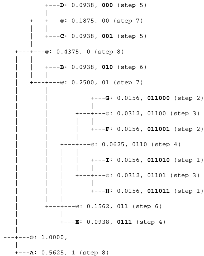
Figure 5.5 Huffman Tree: Product code.
