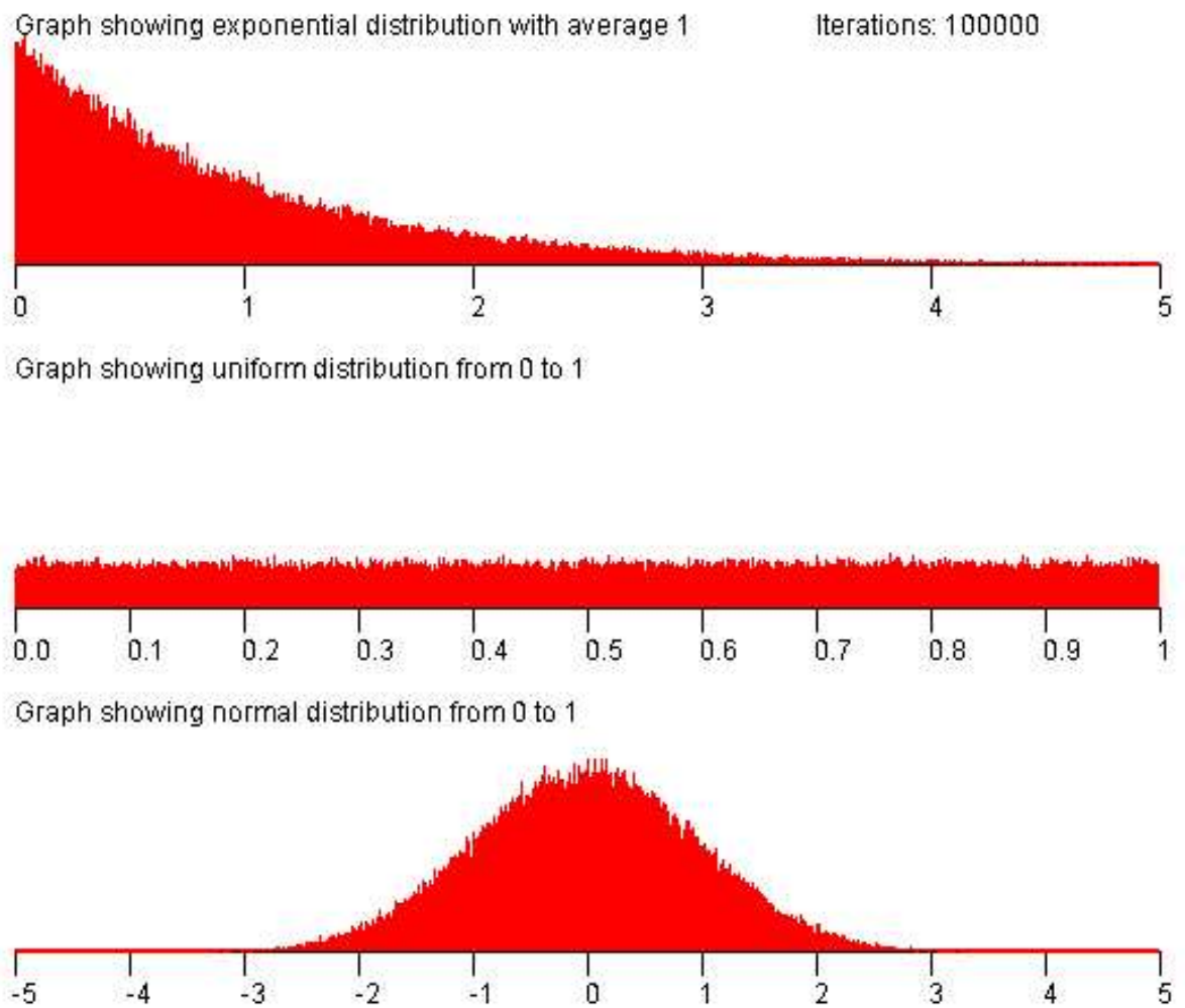
Figure 16.3 Plot of 100000 Points in Three Distributions.
