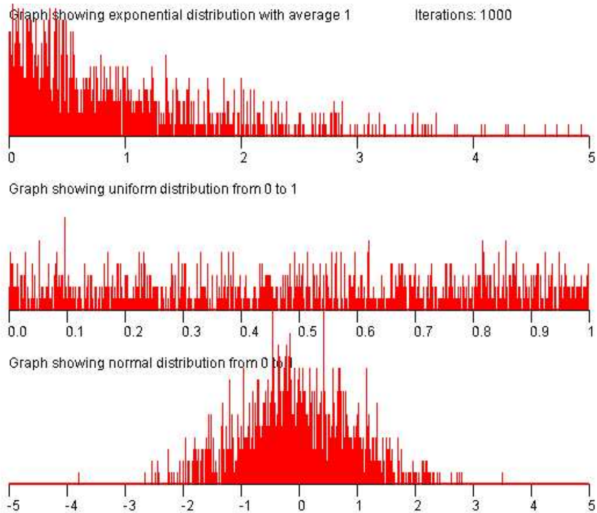
Figure 16.1 Plot of 1000 Points in Three Distributions.
