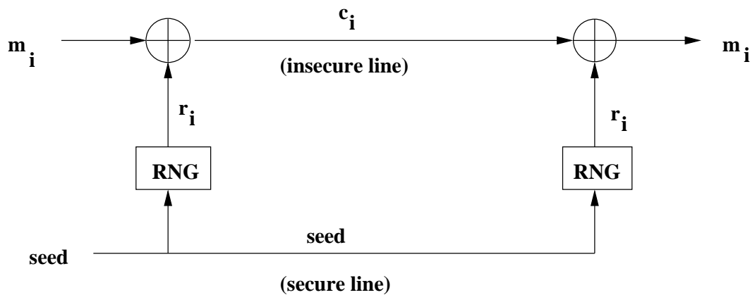
Figure 1.1 Cryptosystem Using XOR.
