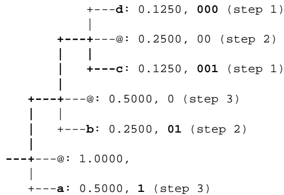
Figure 5.3 Huffman Tree: Decoding.
