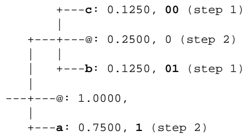
Figure 5.4 Huffman Tree: Entropy less than average code length.
