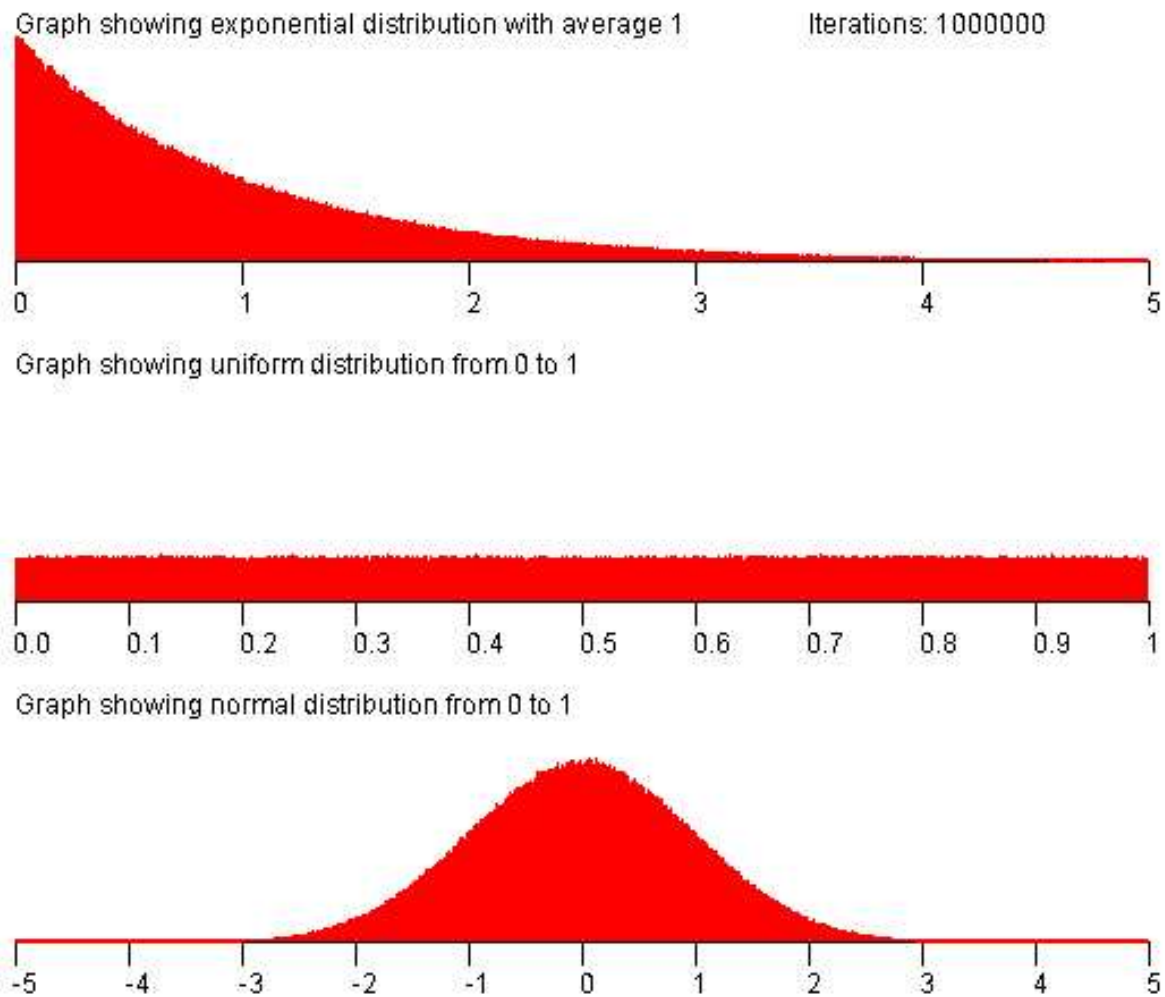
Figure 16.4 Plot of 1000000 Points in Three Distributions.
