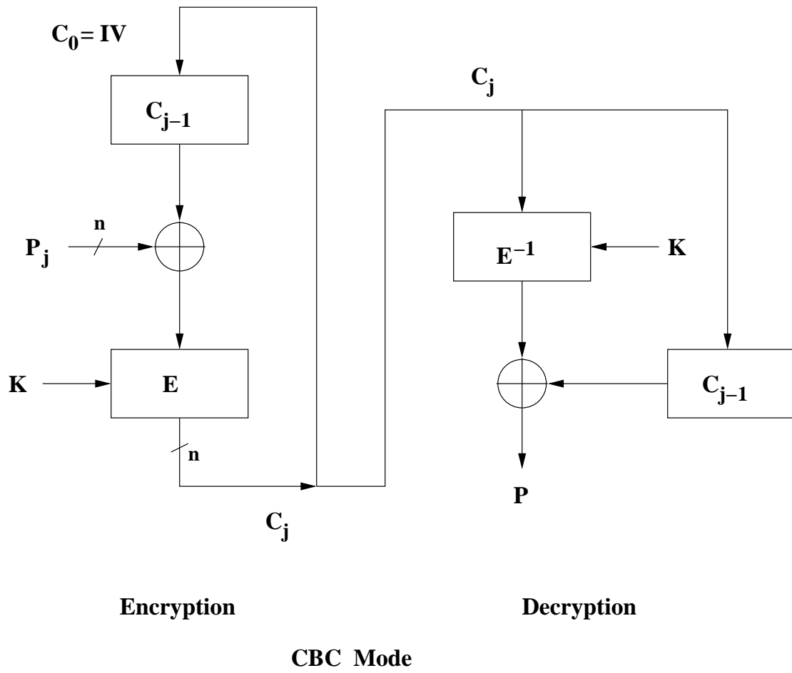
Figure 11.1 The Cipher Block Chaining Mode.
