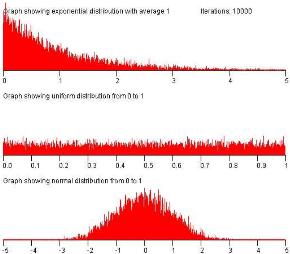
Figure 16.2 Plot of 10000 Points in Three Distributions.
